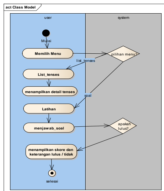
Gambar 2. Activity Diagram
