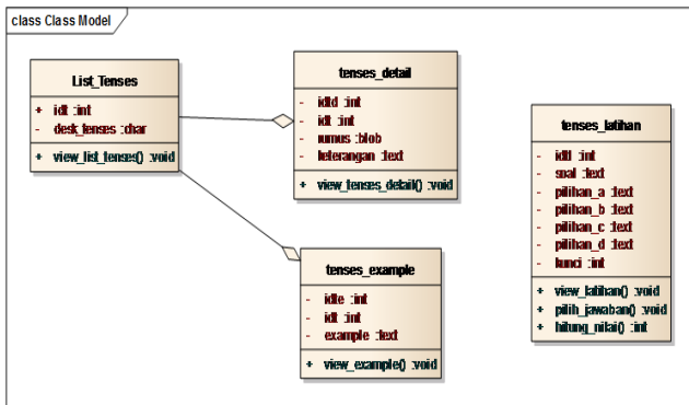
Gambar 3. Class Diagram
